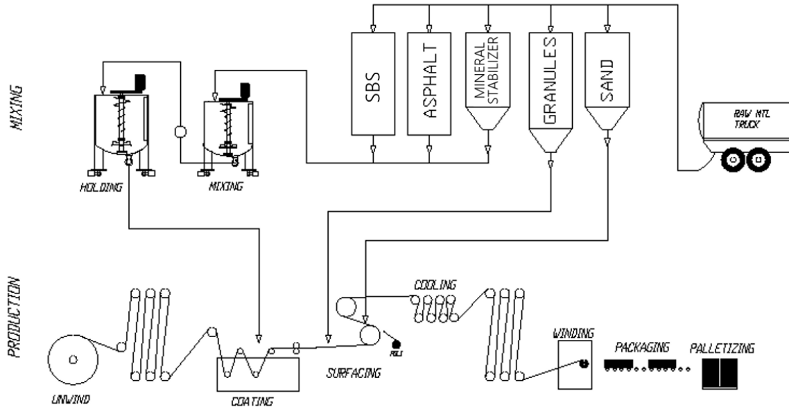
Figure 1: Modified bitumen sheet process diagram
