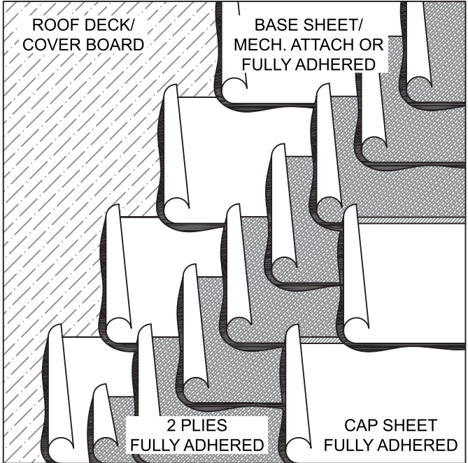
Four ply, hot mopped, built-up roofing system with a fiberglass base, ply, and a high-performance SBS polymer modified fiberglass/poly-ester scrim cap sheet installed over an approved roof deck.
