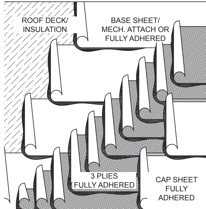
Five-ply, hot mopped, built-up roofing system with conventional fiber-glass base/ply sheets and a highly-reflective, factory coated SBS cap sheet installed over an approved roof deck.
