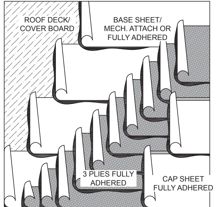
Five ply, hot mopped, built-up roofing system with conventional fiber-glass base, ply, and cap sheet installed over an approved roof deck.
