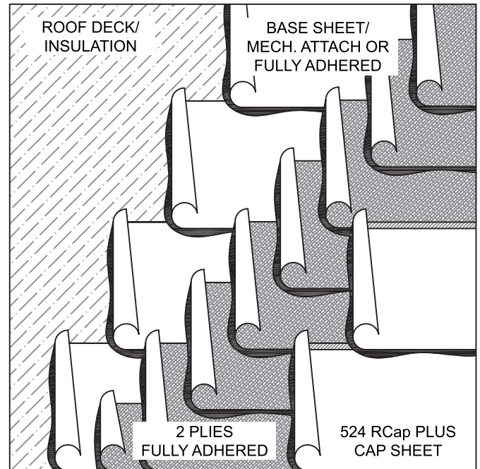
Four-ply, hot mopped, built-up roofing system with SBS fiberglass base/ply sheets and a highly-reflective, factory coated cap sheet installed over an approved roof deck.
