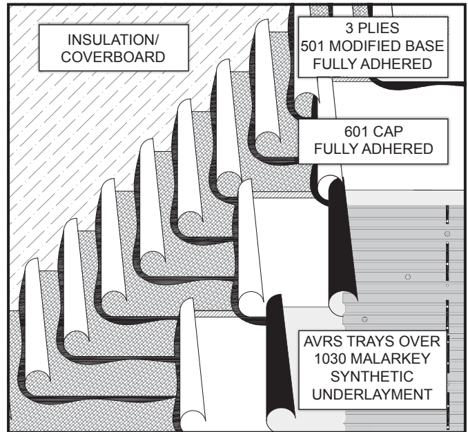
Four-ply built-up roofing system (SEBS hot mopped SBS-modified ply and cap sheets) with a synthetic underlayment liner and vegetative roof system installed over an approved roof deck with insulation and coverboard .
