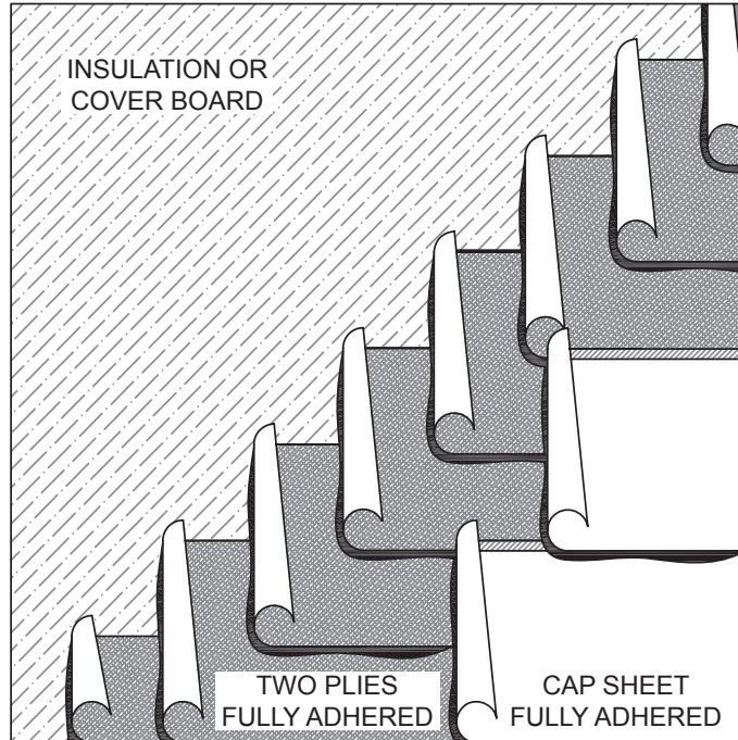
Three-ply, hot mopped, built-up roofing system with conventional fiberglass ply sheets and a SBS modified cap sheet installed over an approved roof deck.
