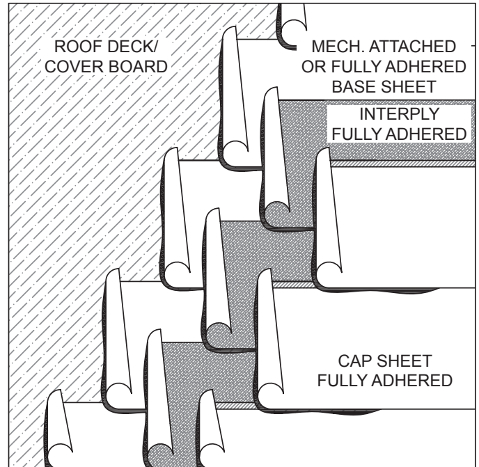
Three ply, hot mopped, built-up roofing system with conventional fiber-glass base, ply, and cap sheet installed over an approved roof deck.
