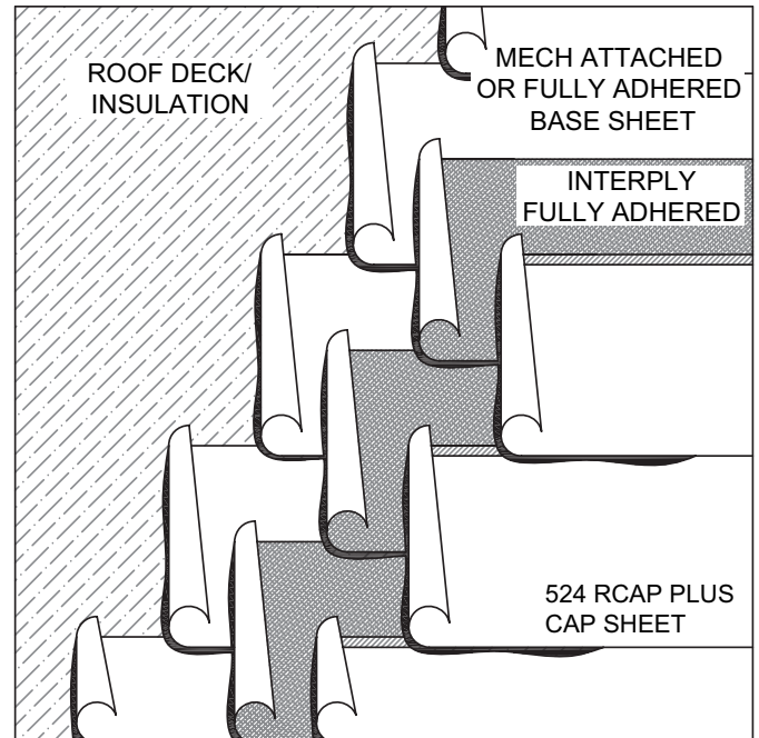
Three-ply, hot mopped*, built-up roofing system with SBS fiberglass base, ply, and a highly-reflective, factory-coated SBS cap sheet installed over an approved roof deck.
